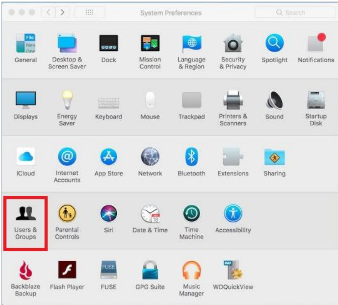
Figure 3. System Preferences
