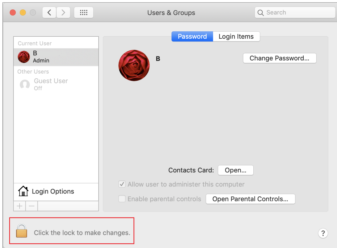
Figure 4. Users & Groups
